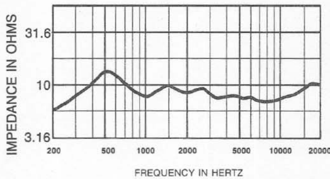
FIGURE 6 Impedance Response — 2-Inch Plane-Wave Tube
