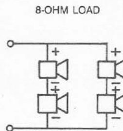
FIGURE 8 Electrical Connections
