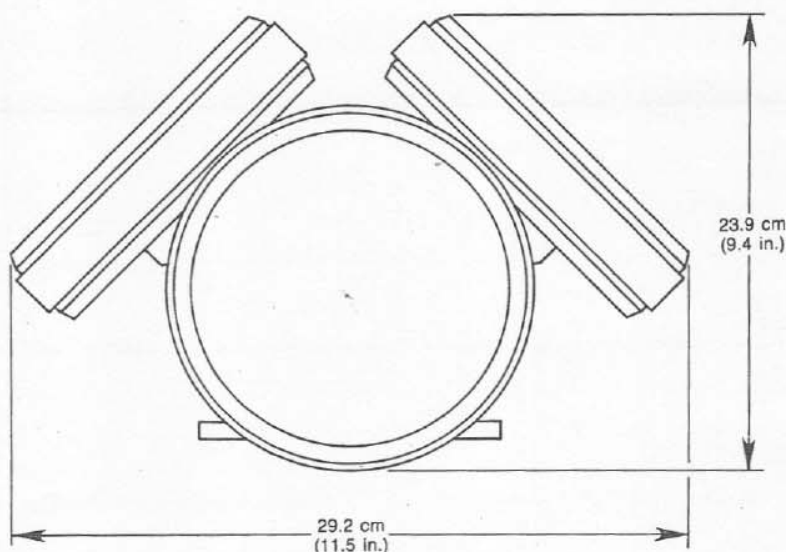
FIGURE 2 Dimensions
